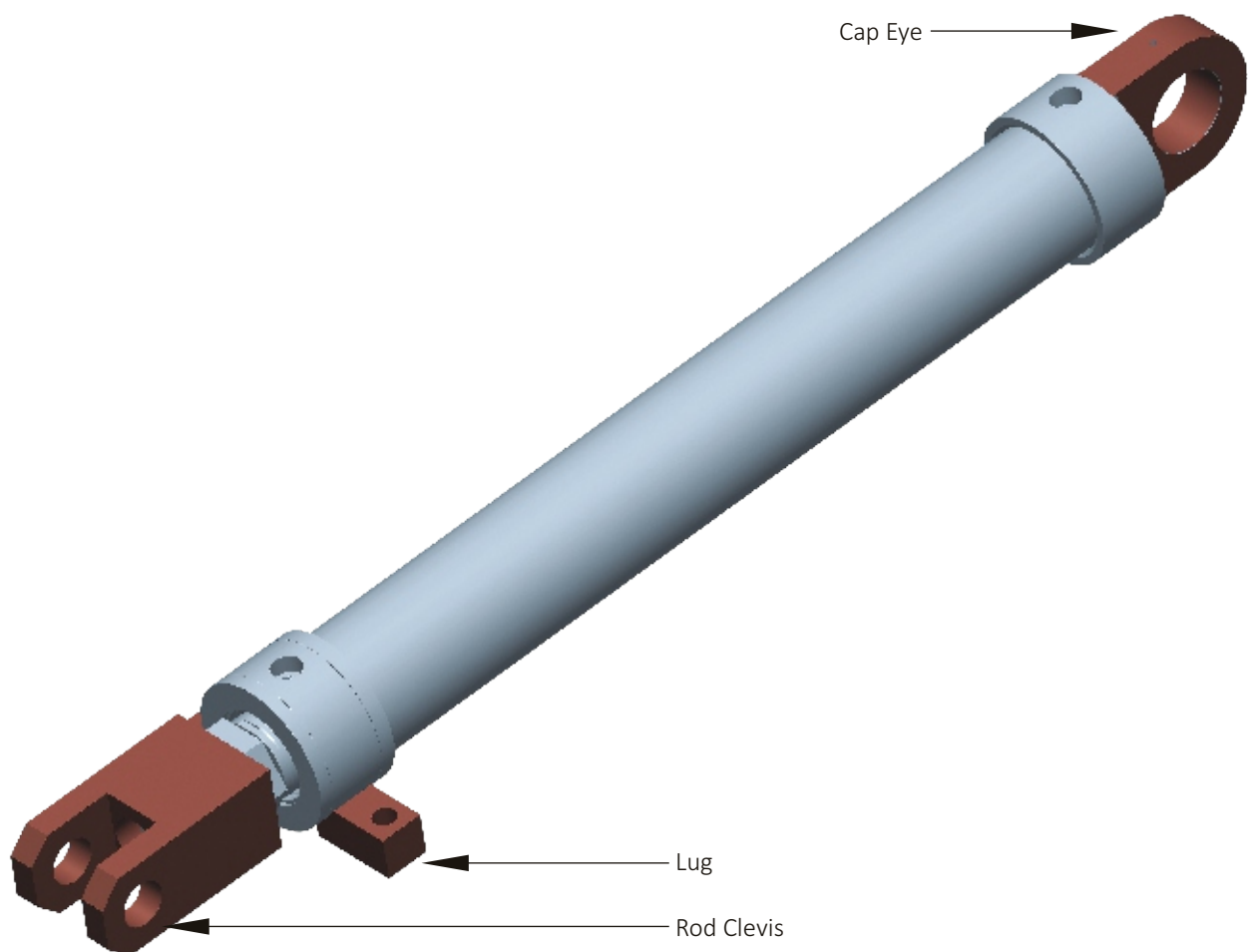
Fig.6 Foot and Clevis mounted Hydraulic cylinder Bore \phi 250mm x Piston Rod \phi 180mm x Stroke 6250 mm manufactured for several steel mills in India and abroad for Roll change application.
