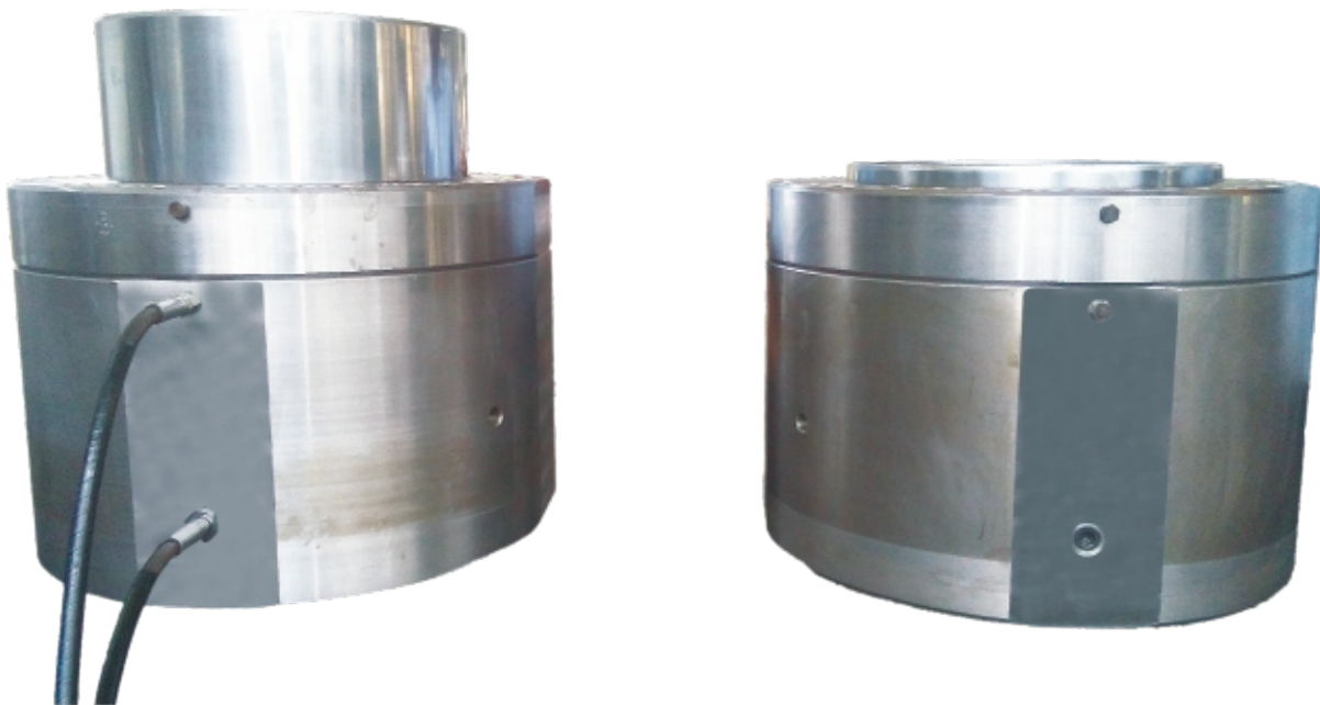
2. Typical View of a Roll Force Cylinders Bore \phi 800mm x Piston Rod \phi 750mm x Stroke 272.5mm under cyclical operation test.
